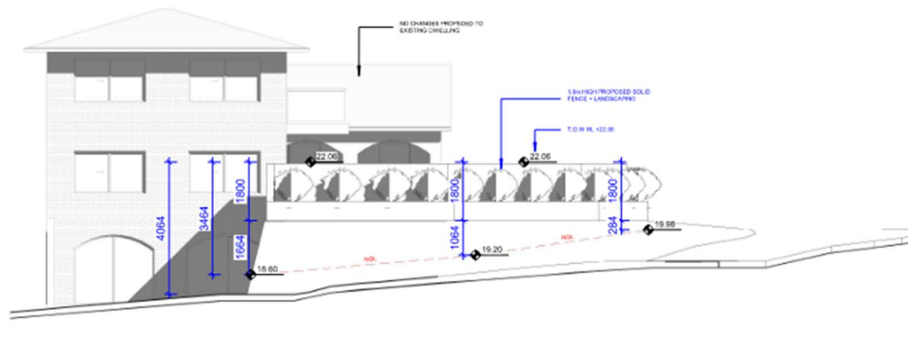
① Street Elevation 01 1 : 100
